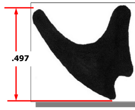
#G (009-344) For 1/8" Fixed glass rubber Sold per foot Black or White
